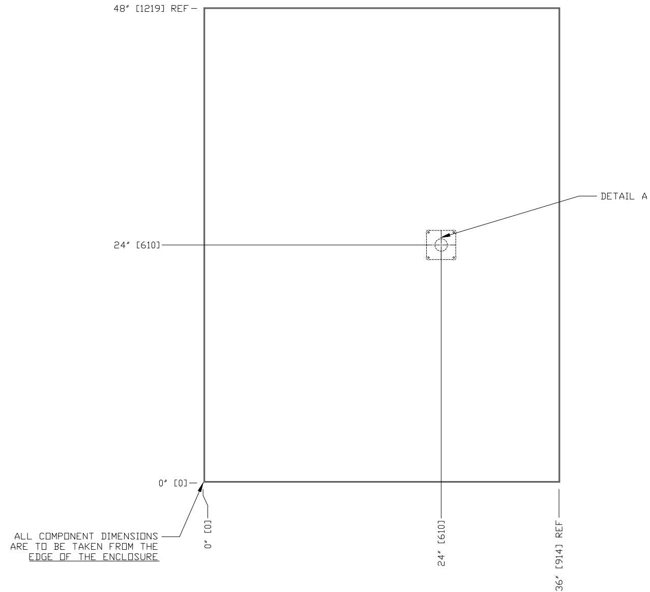
PANEL DETAIL
